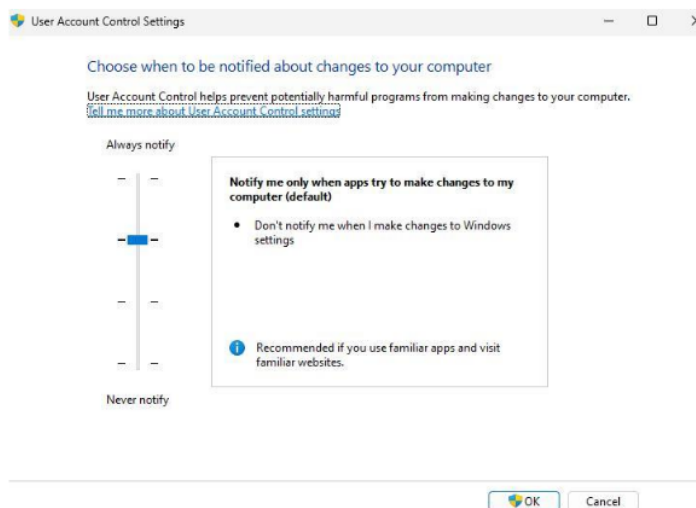
Gambar 4.6 tampilan UAC
