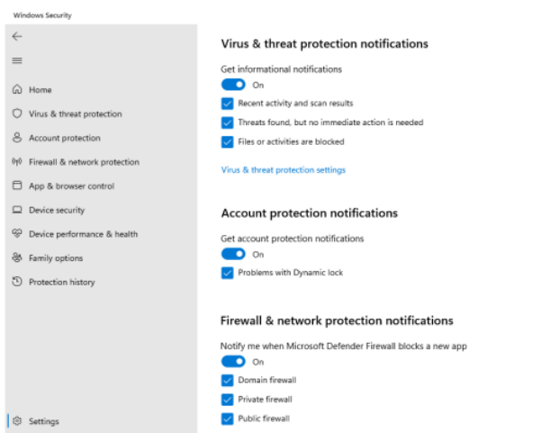
Gambar 4.4 tampilan UX
