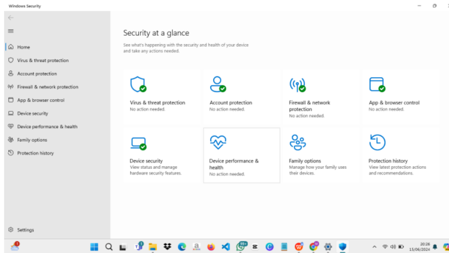
Gambar 4.2 tampilan UI
