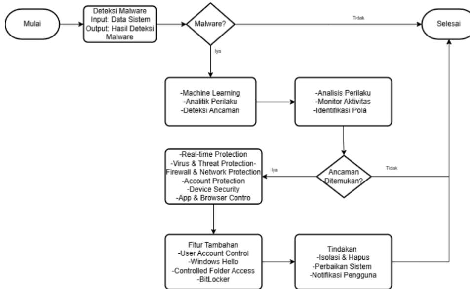
Gambar 4.1 flowchart
