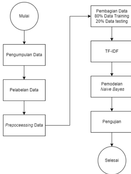
Gambar 1. Flowchart
