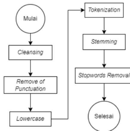
Gambar 2. Flowchart Preprocessing
