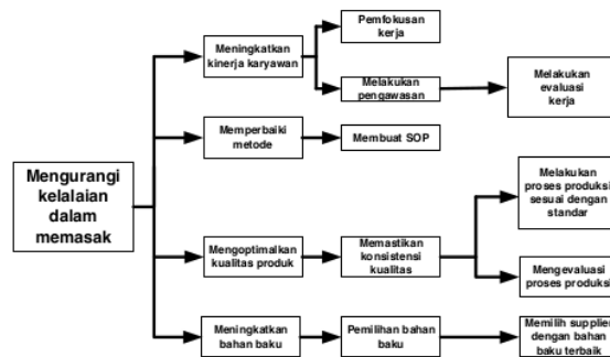
Gambar 7. Tree Diagram
