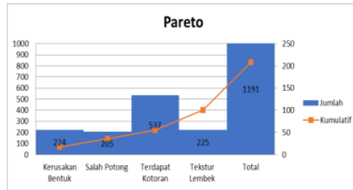
Gambar 1. Diagram Pareto
