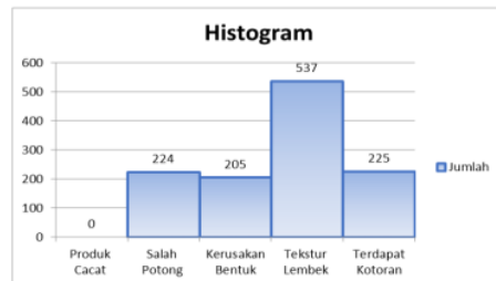
Gambar 2. Diagram Histogram
