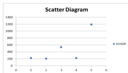
Gambar 3. Scatter Diagram
