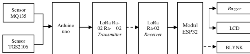
Gambar 3.1 Blok Diagram
