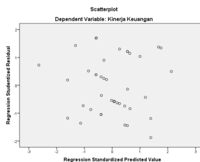
Gambar 2. Hasil Scatterplot
