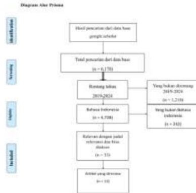
22 Gambar 1. Diagram Prisma
